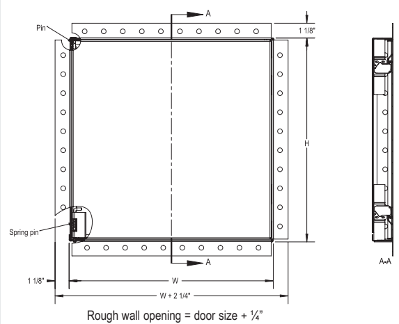
Rough wall opening = door size + 1/4"
