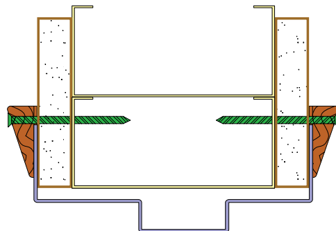
Metal Stud Application
