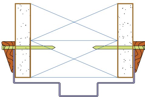
Wood Stud Application
