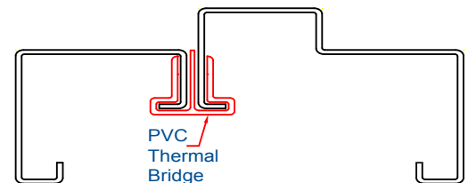
Thermal Break Double Rabbet Profile
