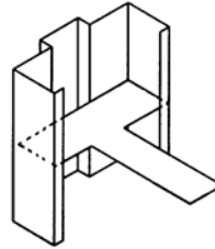
MTA Masonry "T"
